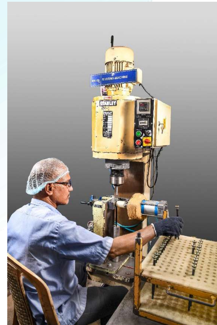
PISTON ROD RIVETTING
